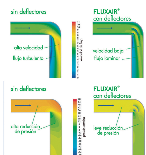
CODO VERTICAL
